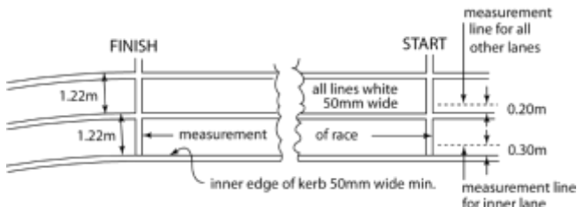
Figure TR14 - Track measurements (infield view)
